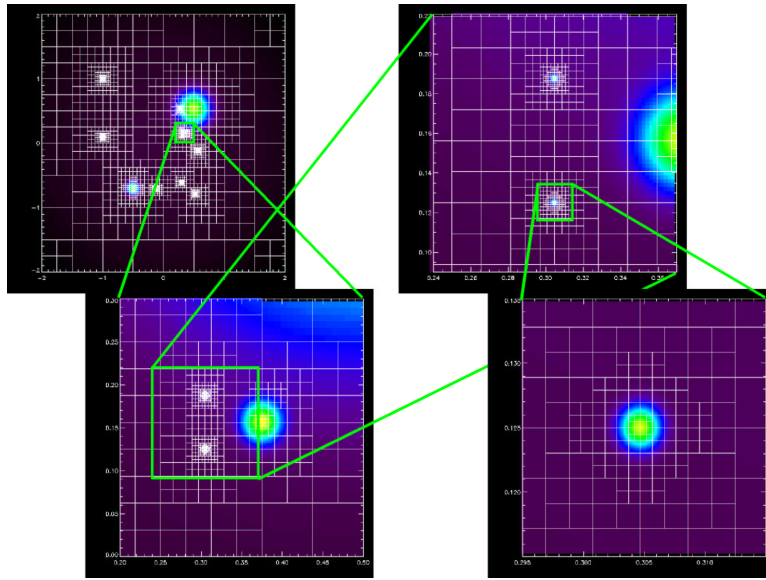
Figure 16.30: Density field and block structure for a 14-level mesh applied to the Huang-Greengard test problem. The effective resolution of the mesh is 65,536^2 .
