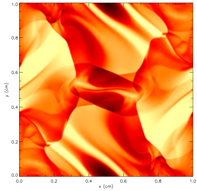
Figure 16.25: Density contours in the Oszag-Tang MHD vortex problem at t = 0.5 .
