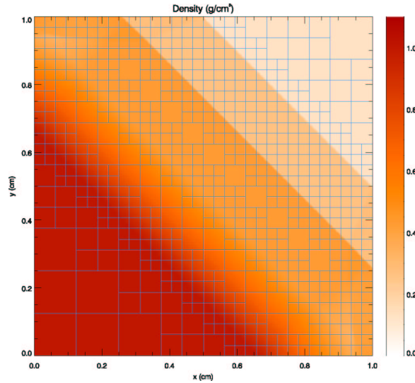
Figure 16.3: Density in the diagonal 2D Sod problem with six levels of refinement at t = 0.2 . The outlines of AMR blocks are shown (each block contains 8 \times 8 zones).
