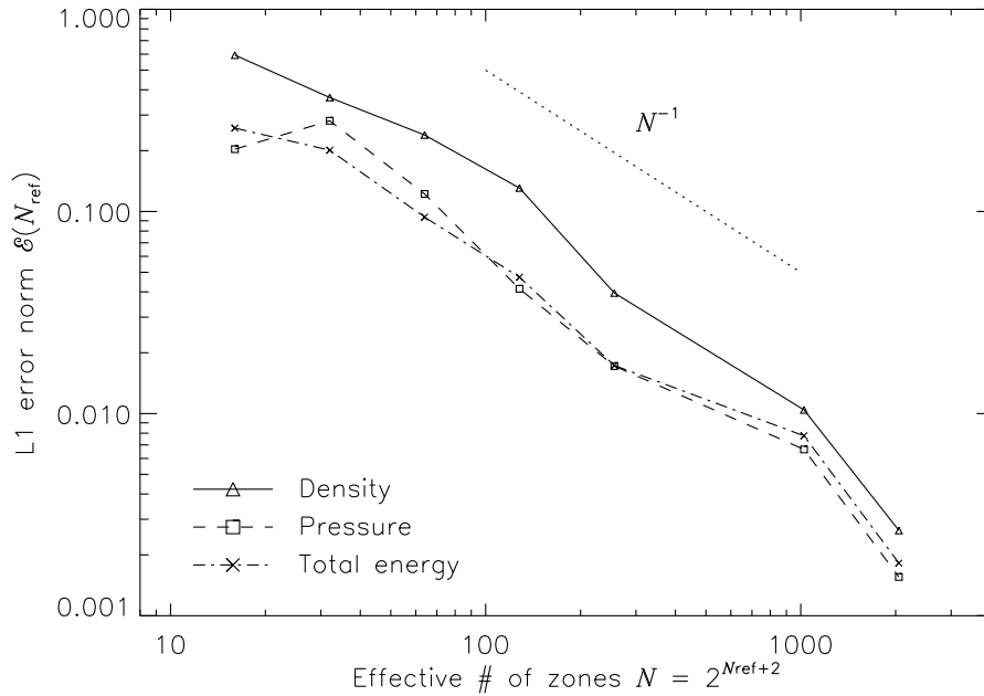
Figure 16.5: Self-convergence of the density, pressure, and total specific energy in the 2blast test problem.
