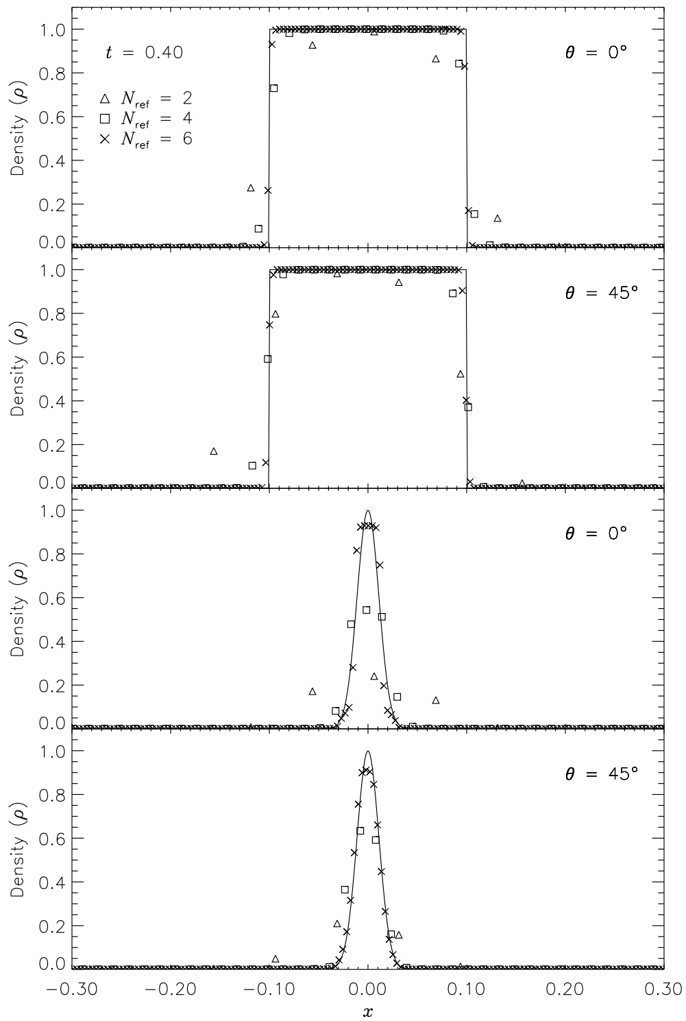
Figure 16.9: Density pulse in the advection tests for 2D grids at t = 0.4 . Symbols represent numerical results using grids with different levels of refinement N_{\text{ref}} (2, 4, and 6).
