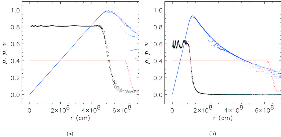
Figure 16.29: Density (black), pressure (red), and velocity (blue) profiles in the homologous dust collapse problem at (a) t = 0.0368 sec and (b) t = 0.0637 sec. The density, pressure, and velocity are scaled as discussed in the text.
