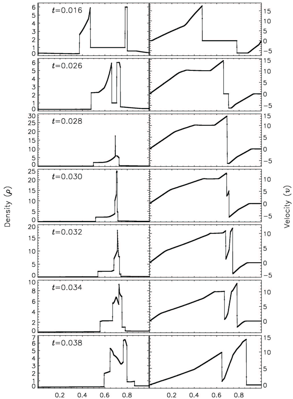
Figure 16.4: Density and velocity profiles in the Woodward-Colella interacting blast-wave problem, as computed by FLASH using ten levels of refinement.
