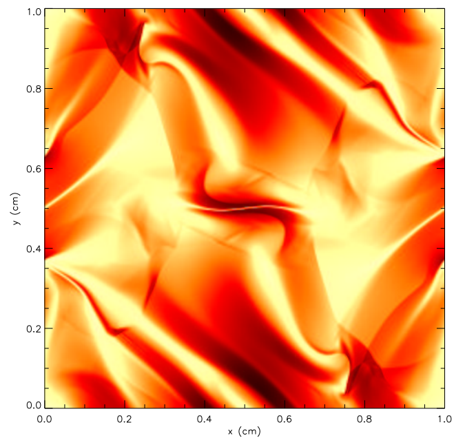
Figure 16.26: Magnetic field contours in the Oszag-Tang MHD vortex problem at t = 0.5 .
