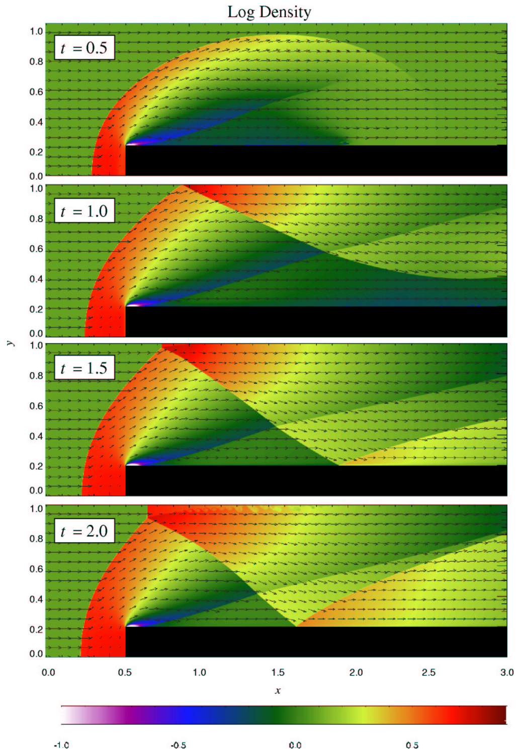
Figure 16.14: Density and velocity in the Emery wind tunnel test problem, as computed with FLASH. A 2D grid with five levels of refinement is used.
