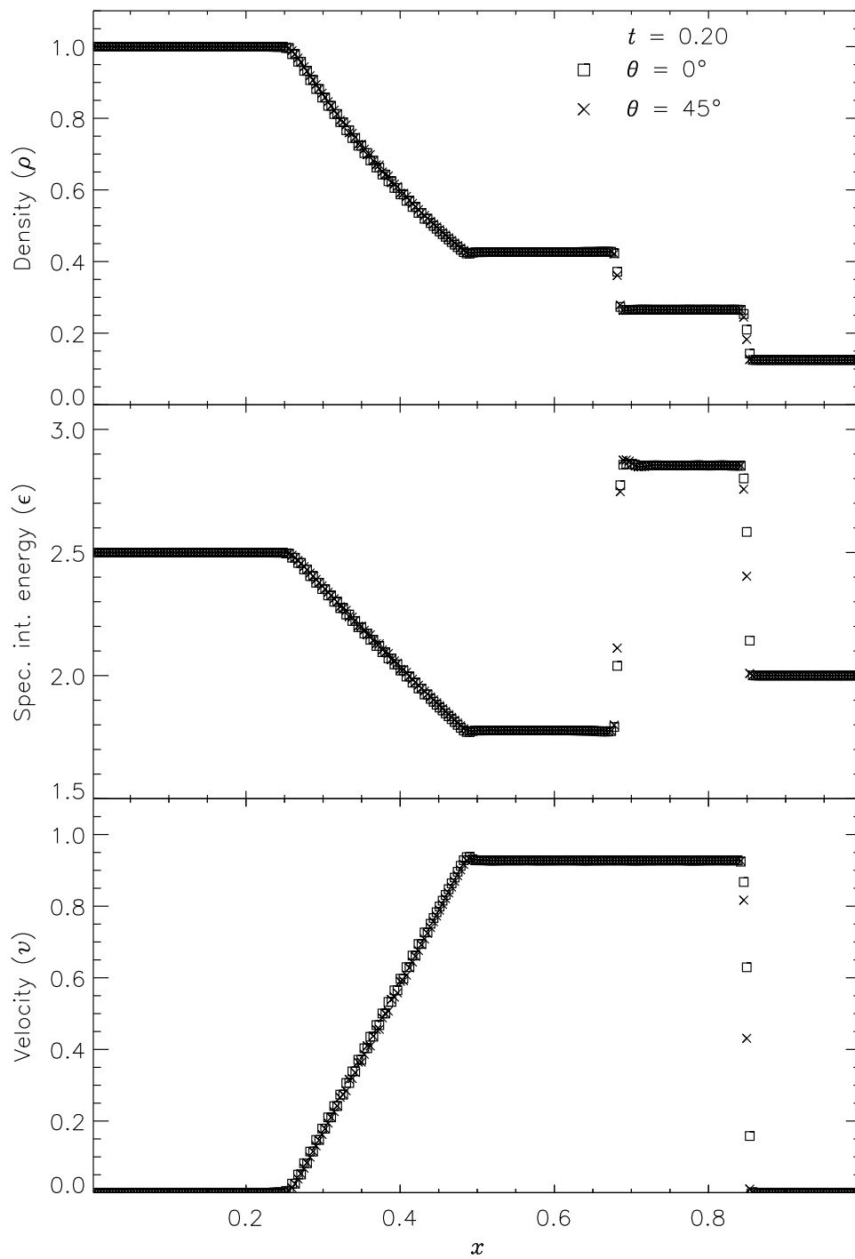
Figure 16.2: Comparison of numerical solutions to the Sod problem for two different angles ( \theta ) of the shock normal relative to the x -axis. A 2D grid with six levels of refinement is used.
