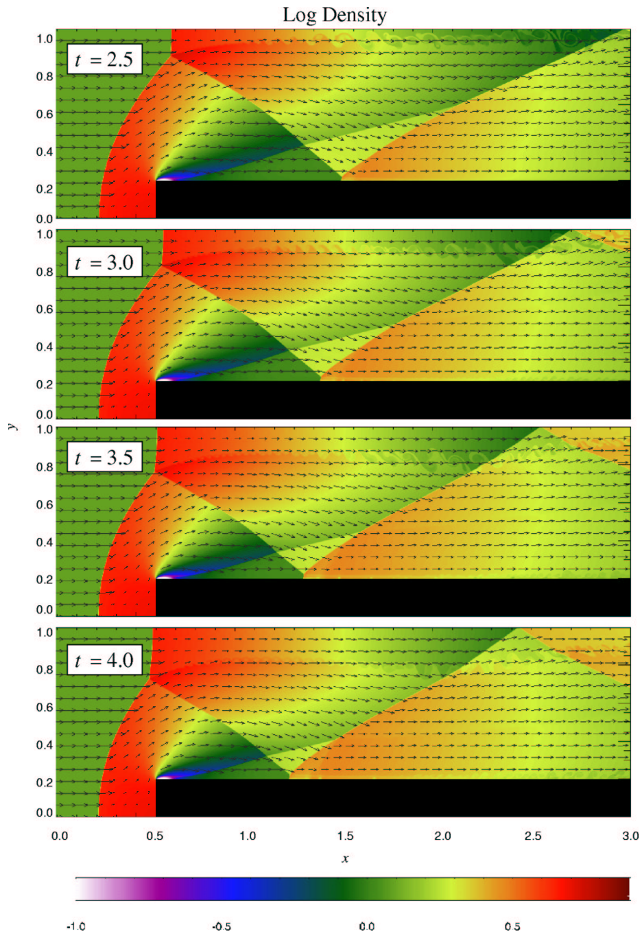
Figure 16.14: Density and velocity in the Emery wind tunnel test problem (continued).
