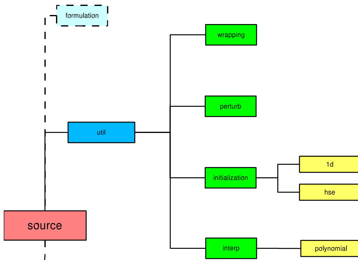
Figure 15.1: The util module directory.
