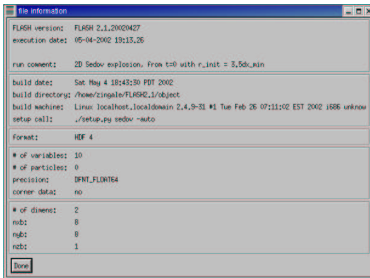
Figure 18.4: The xflash file information widget for the current prototype.
