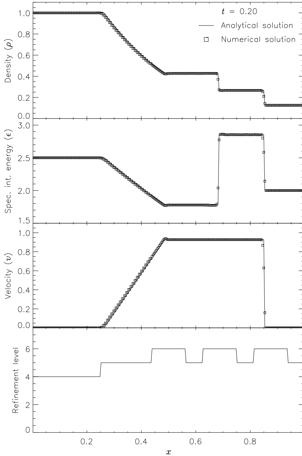
Figure 16.1: Comparison of numerical and analytical solutions to the Sod problem. A 2D grid with six levels of refinement is used. The shock normal is parallel to the x -axis.
