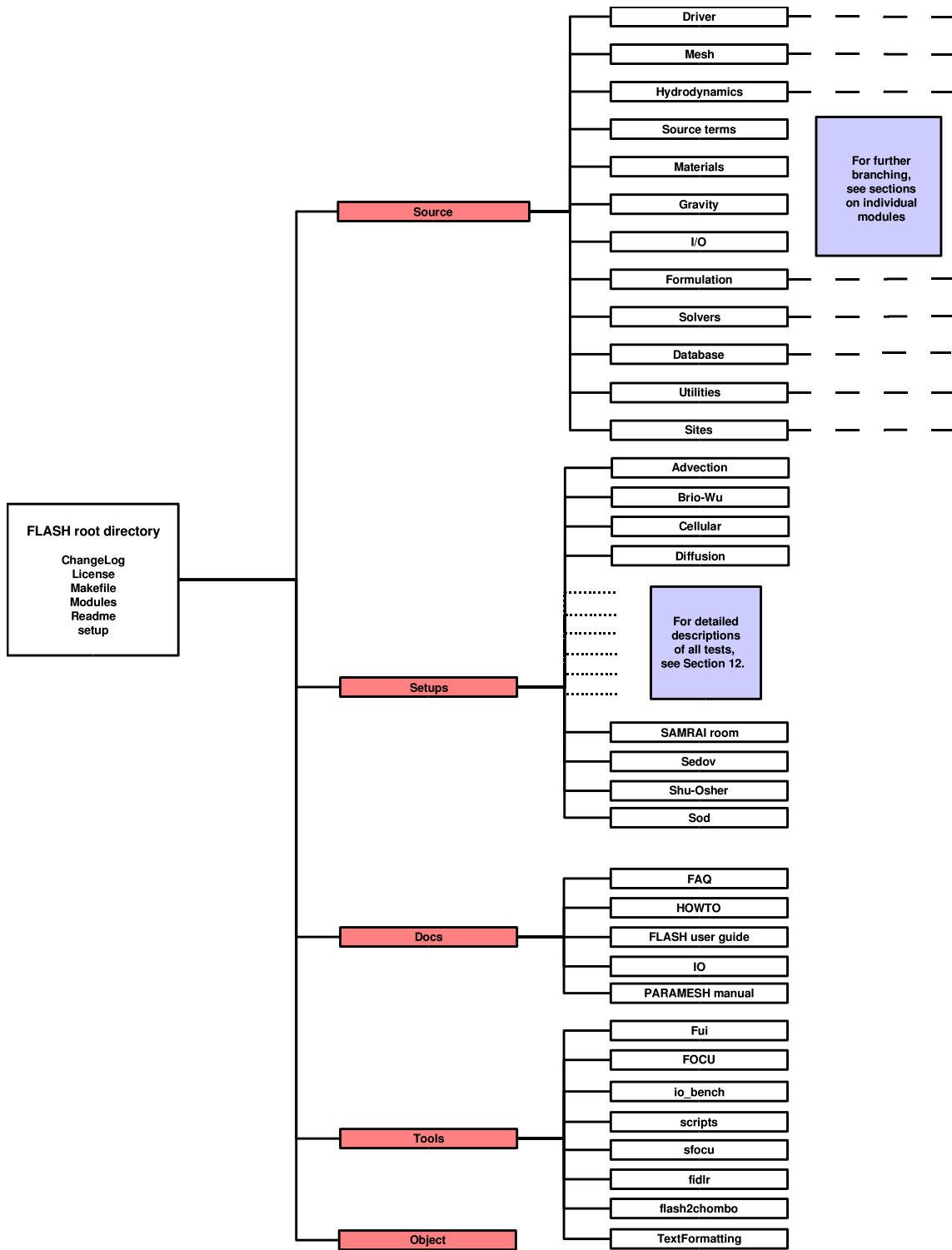
Figure 5.2: Directory structure of FLASH 2.1.
