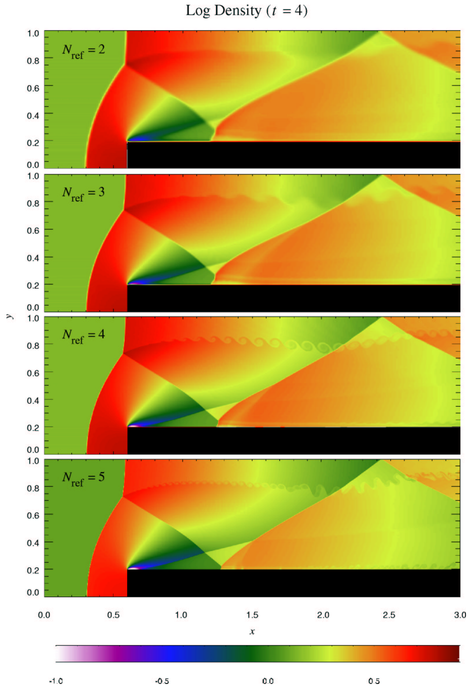
Figure 16.15: Density at t = 4 in the Emery wind tunnel test problem, as computed with FLASH using several different levels of refinement.
