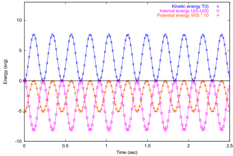
Figure 16.27: Kinetic, internal, and potential energy versus time for a stable Jeans mode with k = 10.984 . Points indicate numerical values found using FLASH 2.0 with a four-level uniform grid. The analytic solution for each form of energy is shown using a solid line.
