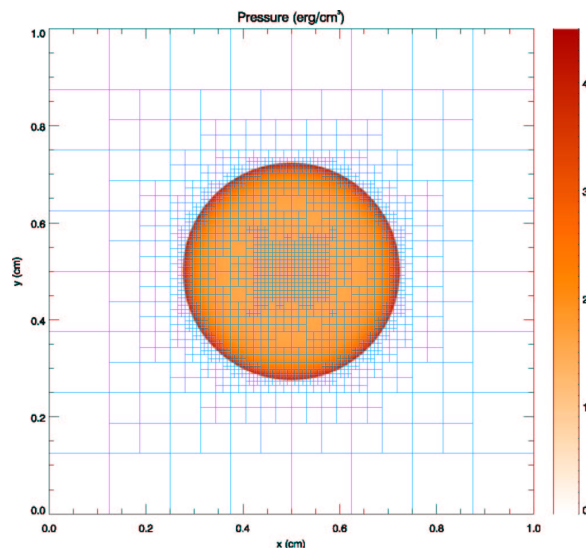
Figure 16.7: Pressure field in the 2D Sedov explosion problem with 8 levels of refinement at t = 0.05 . Overlaid on the pressure colormap are the outlines of the AMR blocks.
