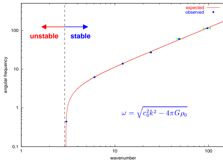
Figure 16.28: Computed versus expected Jeans dispersion relation (for stable modes) found using FLASH 1.62 with a six-level uniform grid.
