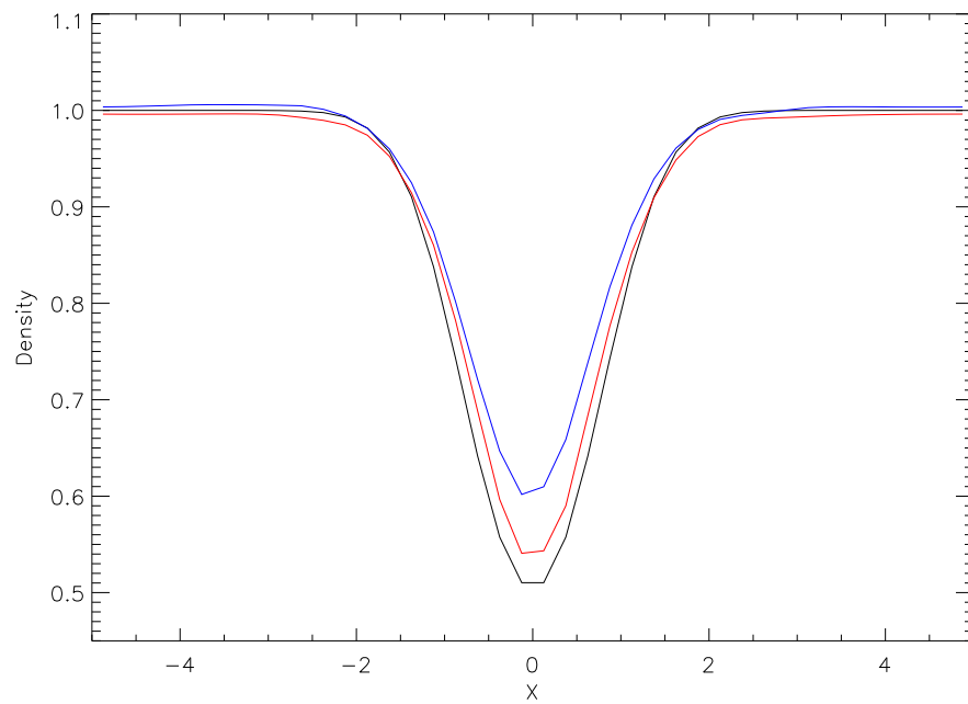
Figure 16.13: Representative density profiles for the isentropic vortex near y = 0.0 at t = 0.0 (black), t = 50.0 (red), and t = 100.0 (blue).
