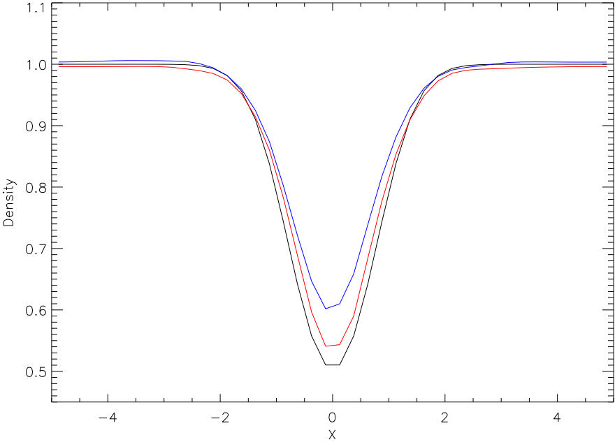
Figure 18.13: Representative density profiles for the isentropic vortex near y = 0.0 at t = 0.0 (black), t = 50.0 (red), and t = 100.0 (blue).
